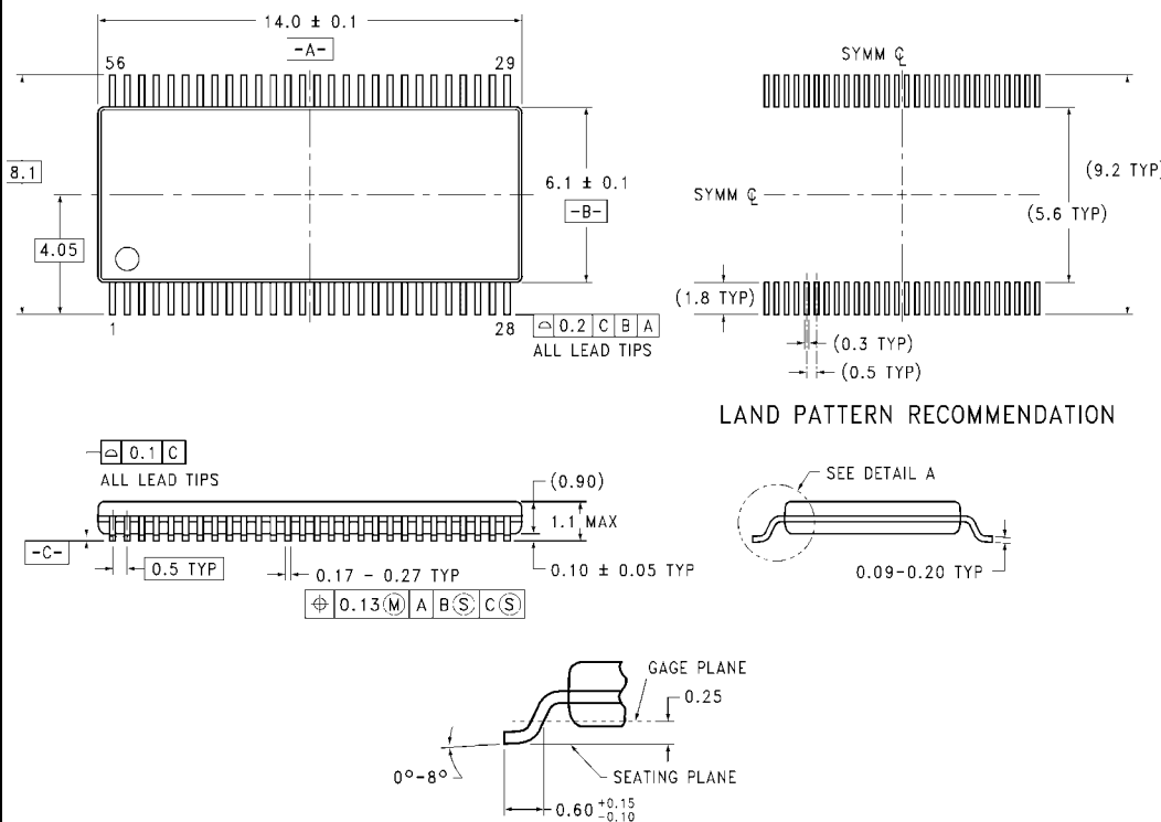
DETAIL A
