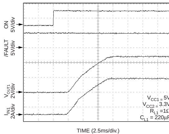
Turn-On (Channel 1)
