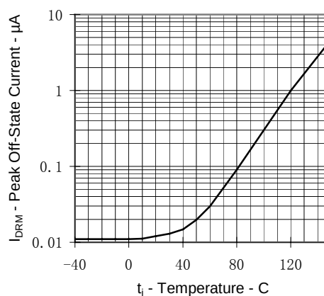
Fig.2 Typical Peak Off-State Current vs Junction Temperature
