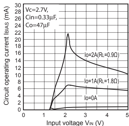
Fig.11 Circuit Operating Current vs. Input Voltage (PQ018EZ02ZxH)
