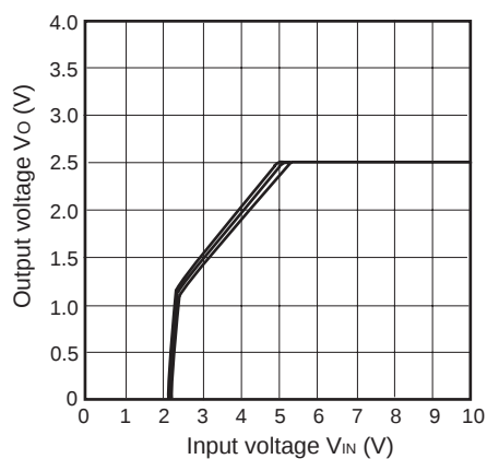
Fig.9 Output Voltage vs. Input Voltage (PQ025EZ02ZxH)
