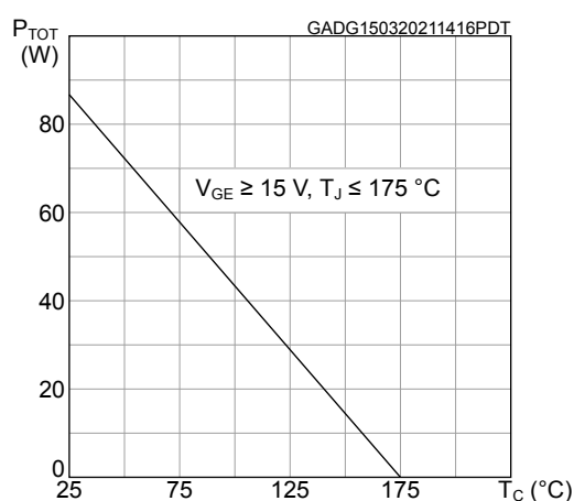
Figure 8. Power dissipation vs case temperature for TO-3PF
