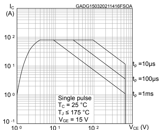
Figure 10. Forward bias safe operating area for TO-3PF
