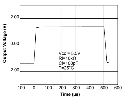
Figure 31. Large signal
