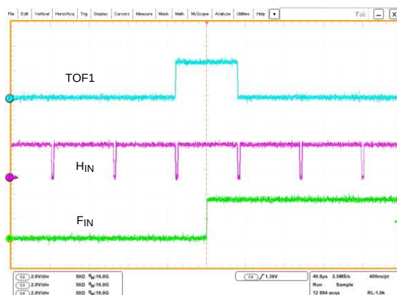
Figure 14. TOF1 Timing
