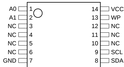
14-Pin TSSOP
