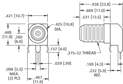
Mounting Detail
