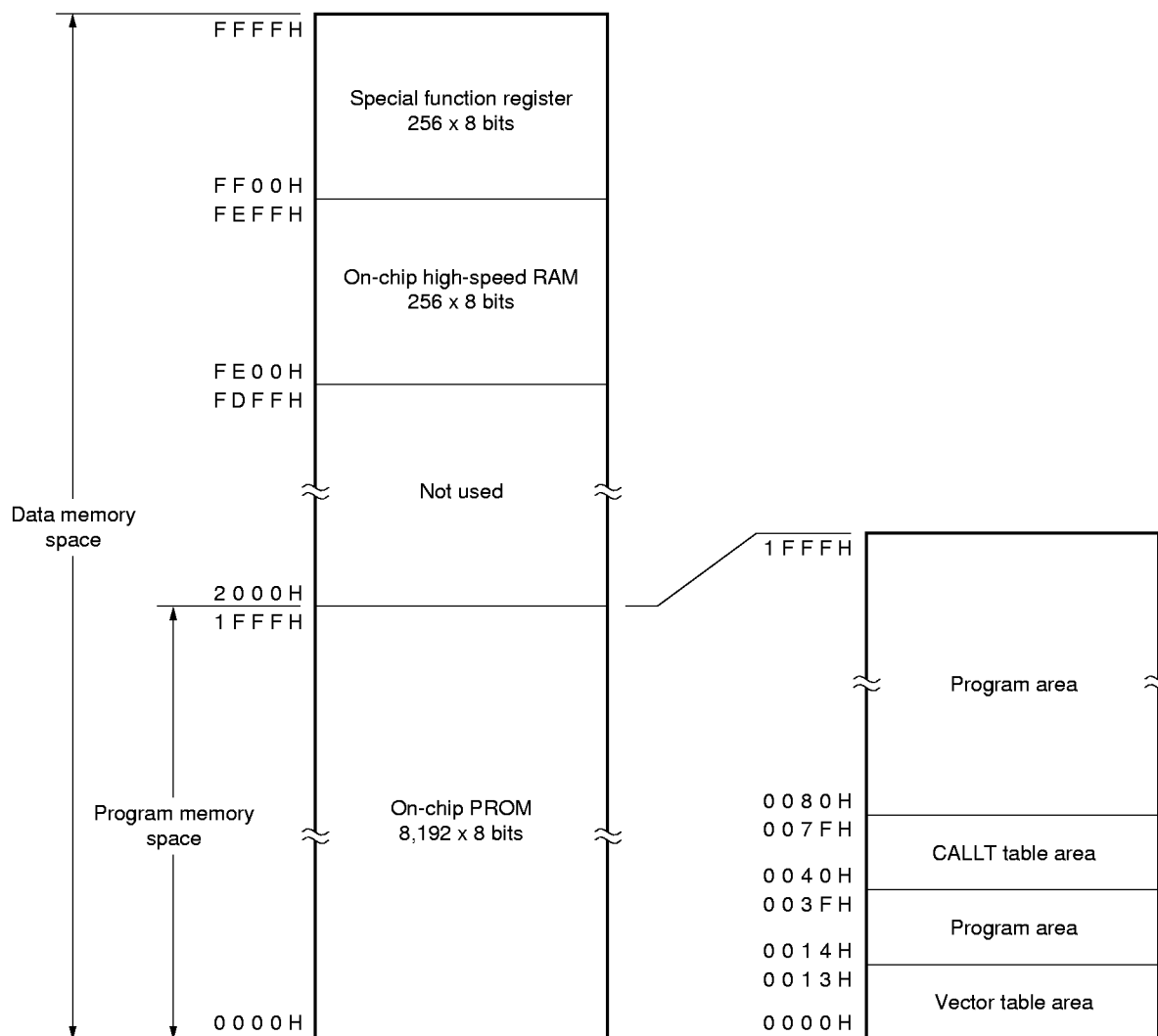
Figure 5-1. Memory Map
