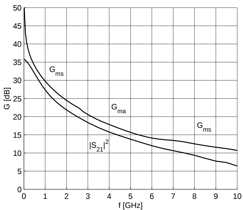
Figure 5-10 Gain G_{ma} , G_{ms} , |S_{21}|^2 = f(f) , V_{CE} = 3 V, I_C = 30 mA
