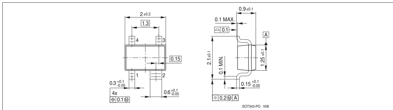
Figure 7-1 Package Outline
