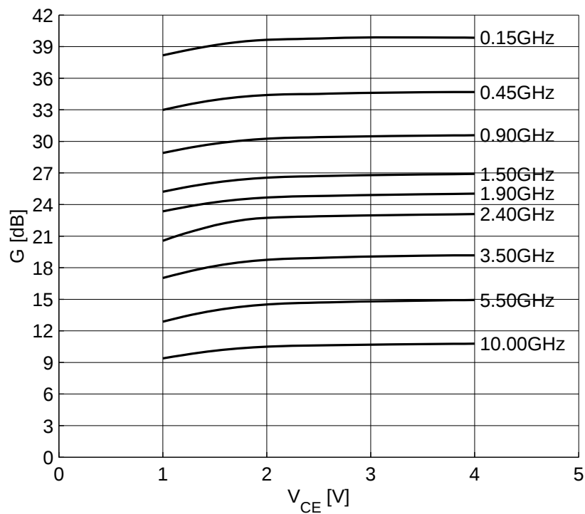
Figure 5-12 Maximum Power Gain G_{\max} = f(V_{CE}) , I_C = 30\text{ mA} , f = \text{Parameter in GHz}
