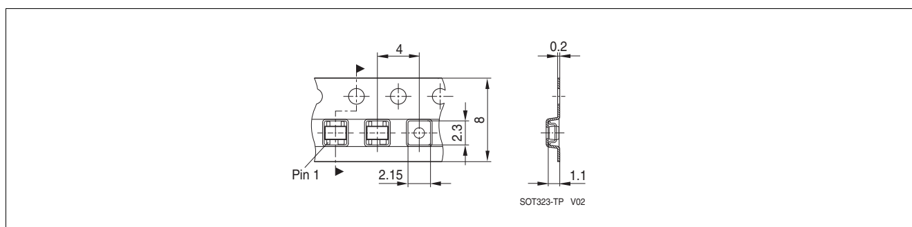
Figure 7-4 Tape Dimensions
