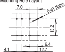
Mounting Hole Layout
