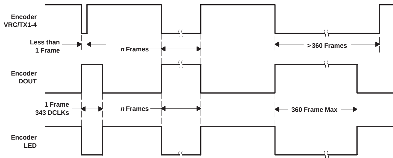
Figure 4. Encoder Timing
