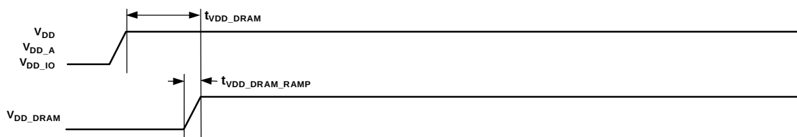
Figure 8. Power-Up Timing
