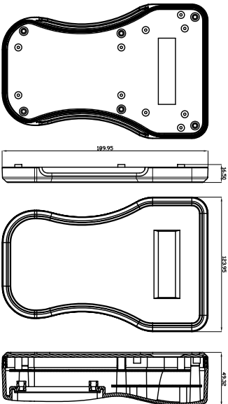
TOP-(MDL-S-16265)
