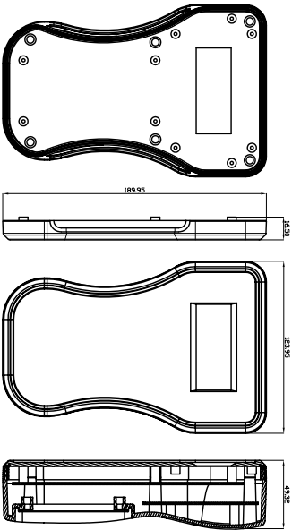
TOP-(MDL-S-16465)
