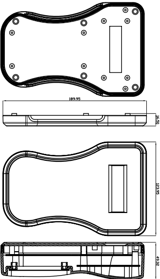
TOP-(MDL-S-16265B)
