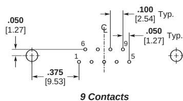
9 Contacts
