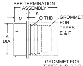
CRIMP KPSE00/MS3120
