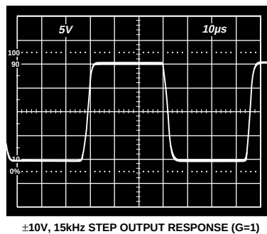
Figure 8. Output Response to Full-Scale Step Input (G = 1 V/V)
