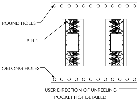
FIG 8 PACKAGING VIEWS
