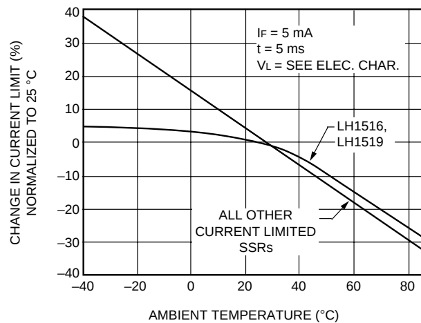
E. Current Limit vs. Temperature
