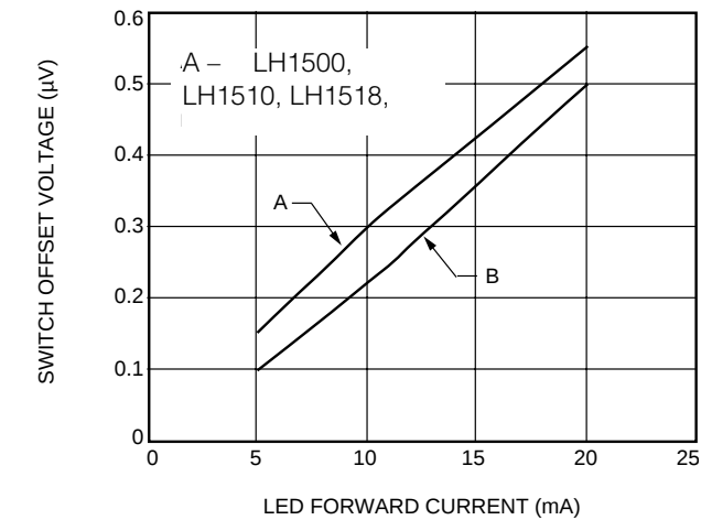
A. Switch Offset Voltage vs. LED Current
