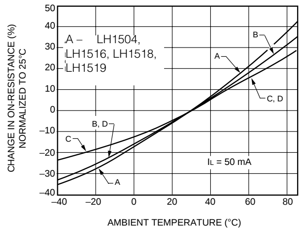
F. ON-Resistance vs. Temperature
