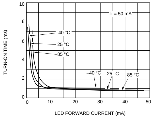
E. Turn-On Time vs. LED Current (LH1510)
