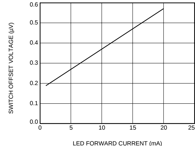
B. Switch Offset Voltage vs. LED Current (LH1525)
