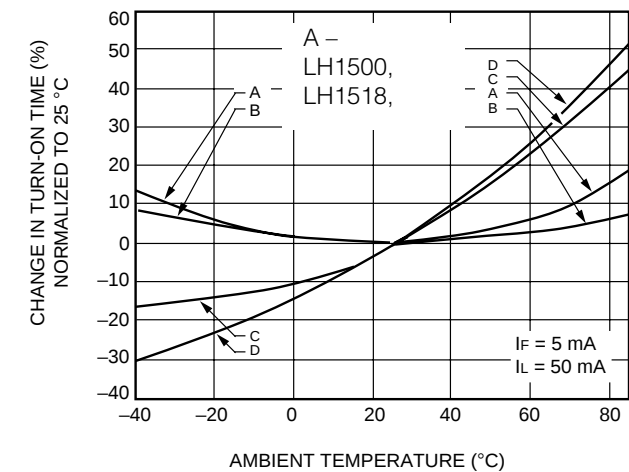
D. Turn-On Time vs. Temperature
