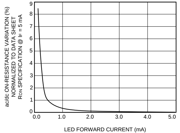
B. Variation in ON-Resistance vs. LED Current (LH1525)
