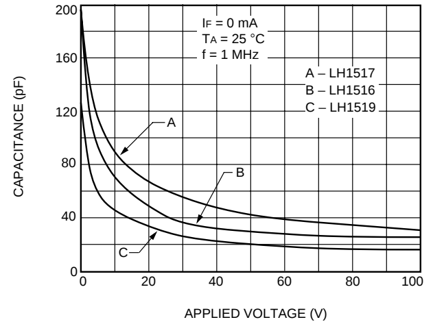
D. Switch Capacitance vs. Applied Voltage
