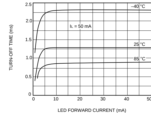
C. Turn-Off Time vs. LED Current (LH1517)
