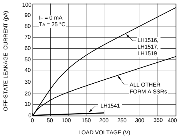
E. Leakage Current vs. Applied Voltage
