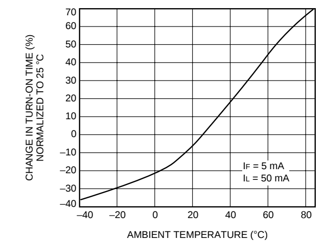
E. Turn-On Time vs. Temperature (LH1541)
