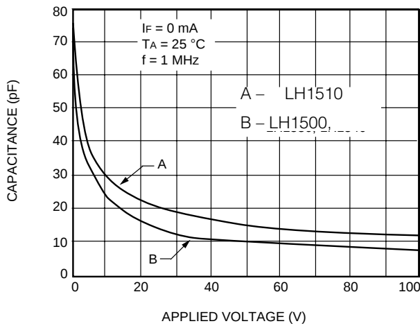
C. Switch Capacitance vs. Applied Voltage
