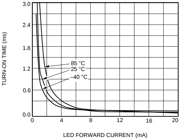
B. Turn-On Time vs. LED Current (LH1525)
