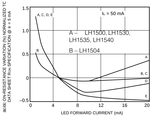
A. Variation in ON-Resistance vs. LED Current
