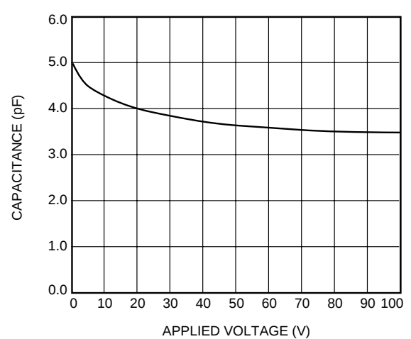
F. Switch Capacitance vs. Applied Voltage (LH1541)
