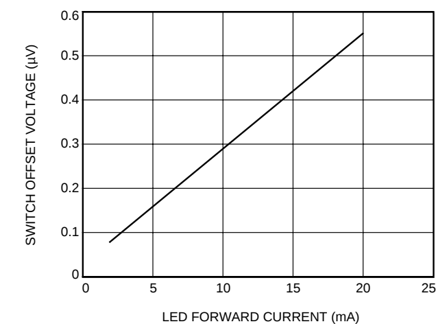
C. Switch Offset Voltage vs. LED Current (LH1541)
