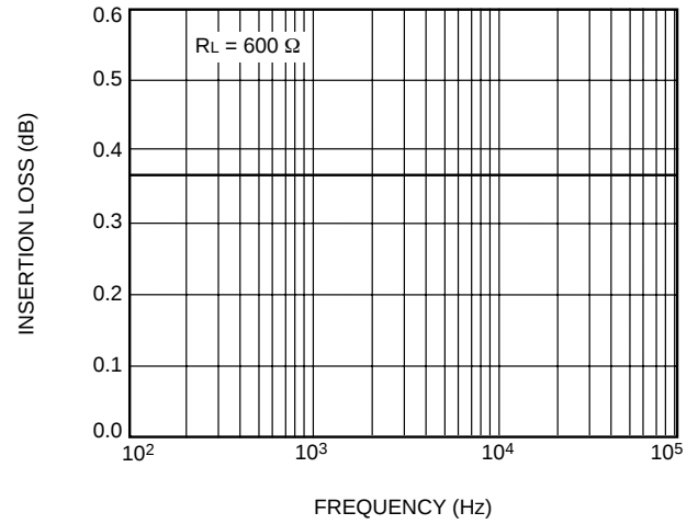
B. Insertion Loss vs. Frequency (LH1525)
