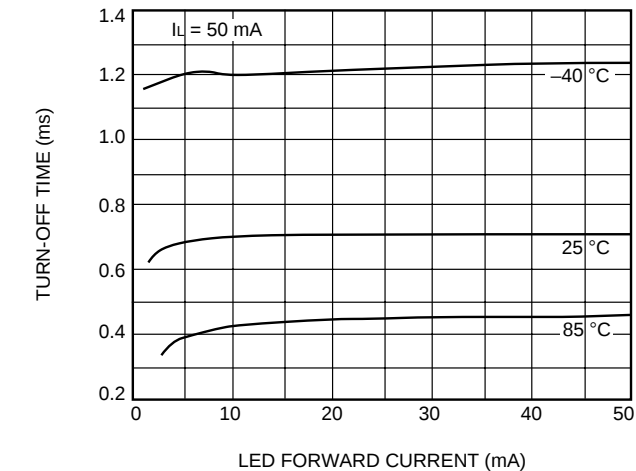
A. Turn-Off Time vs. LED Current (LH1510, LH1518)
