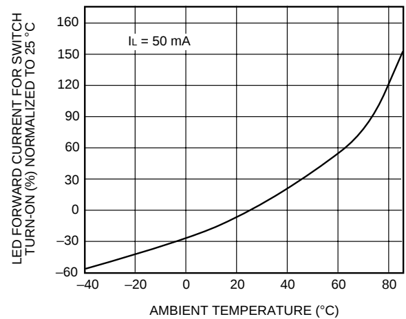
D. LED Current for Switch Turn-On vs. Temperature (LH1541)
