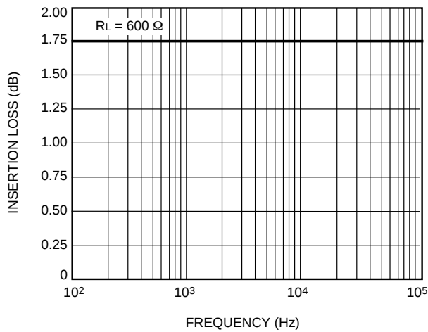
C. Insertion Loss vs. Frequency (LH1541)
