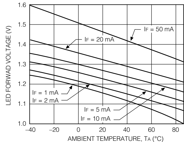
A. LED Voltage vs. Temperature
