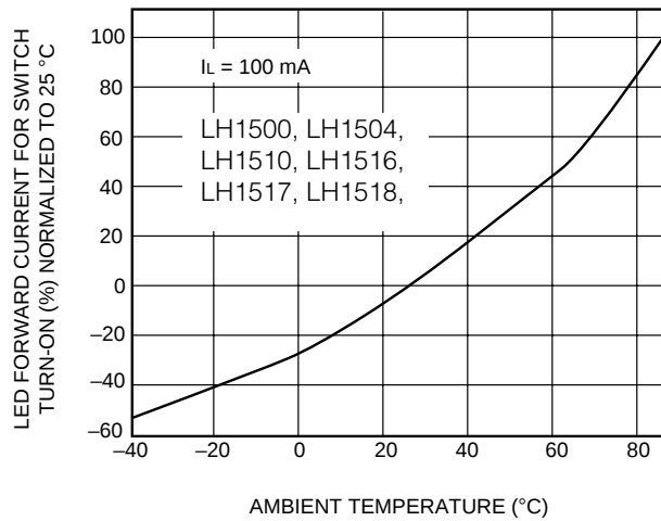
C. LED Current for Switch Turn-On vs. Temperature
