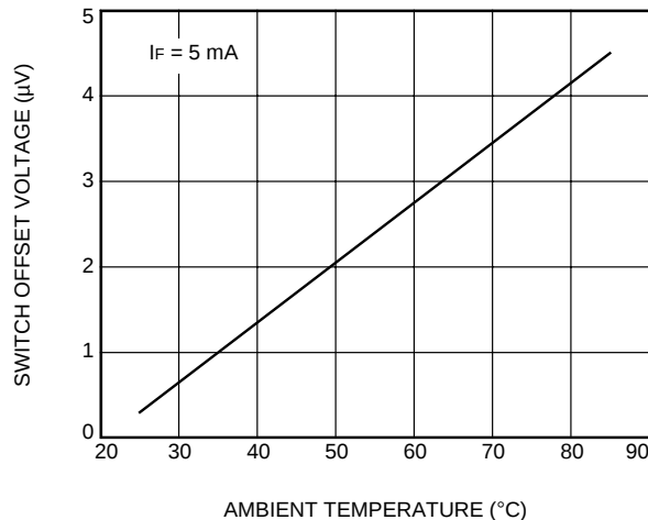
F. Switch Offset Voltage vs. Temperature (LH1525)
