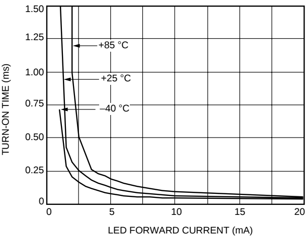
D. Turn-On Time vs. LED Current (LH1541)
