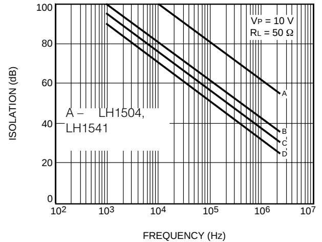
D. Output Isolation
