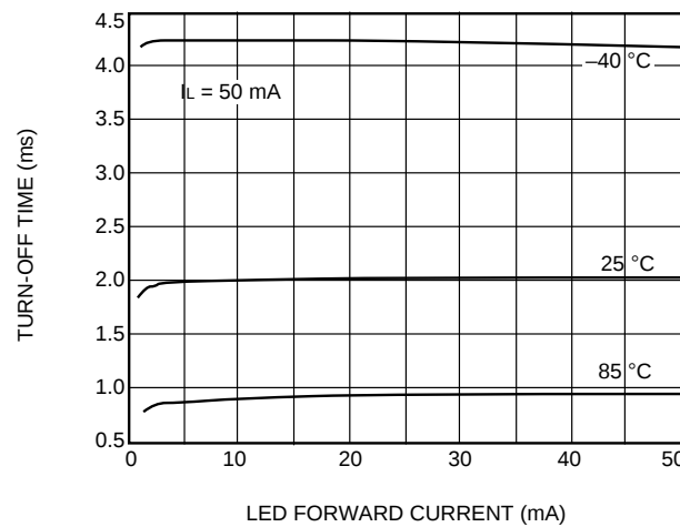
F. Turn-Off Time vs. LED Current (LH1504)
