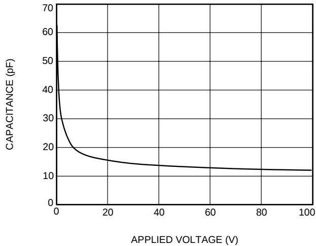
E. Switch Capacitance vs. Applied Voltage (LH1525)
