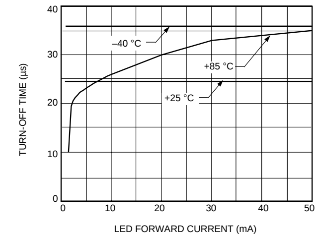
E. Turn-Off Time vs. LED Current (LH1541)
