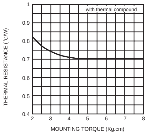
CONTACT THERMAL RESISTANCE \theta_{cf}
