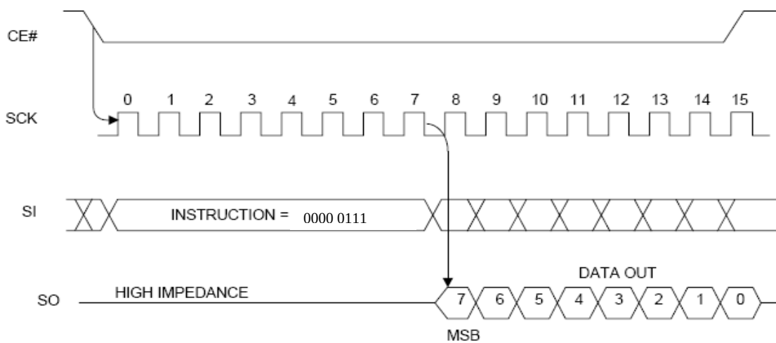
Figure 30. Read Function Register Sequence
