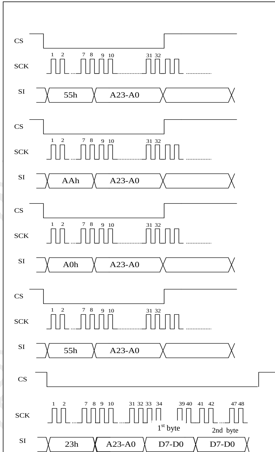
Fig c. program safe guard register
