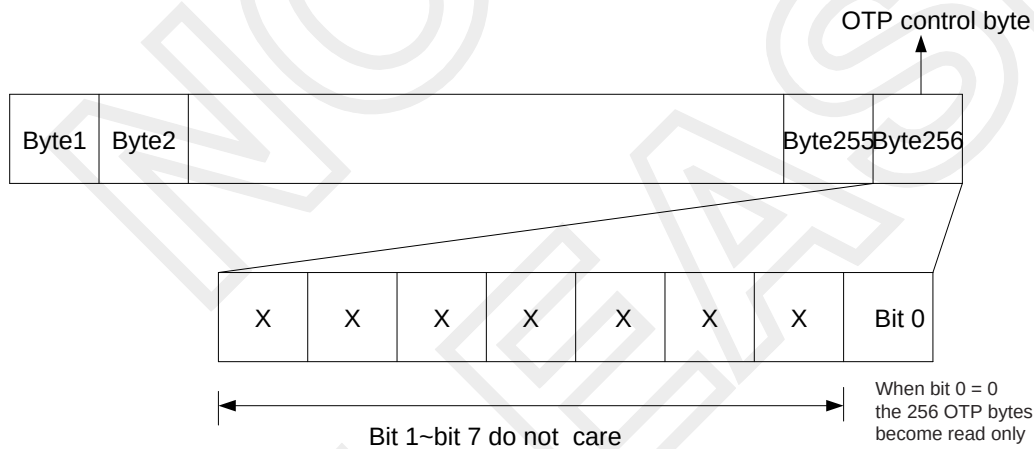
Figure 28. OTP area
