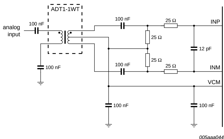
Fig 18. Single transformer configuration suitable for baseband applications
