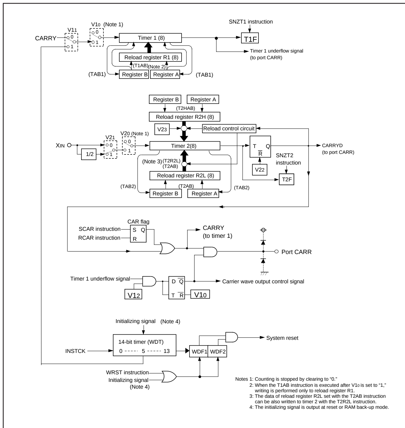
Fig. 13 Timers structure
