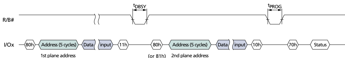
Figure 28: TWO-PLANE PROGRAM PAGE Operation
