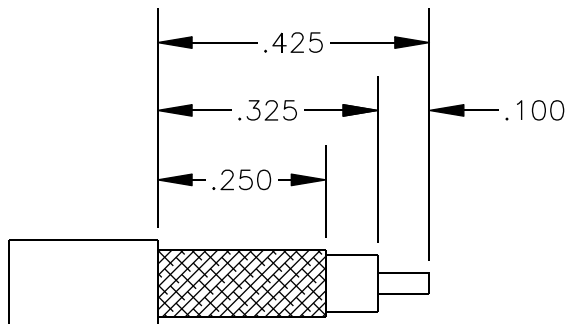
STRIPPING DIMENSIONS
