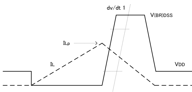
(b) Waveforms
