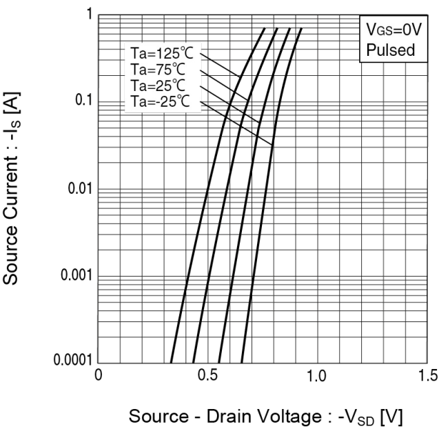
Fig.5 Source Current vs. Source Drain Voltage
