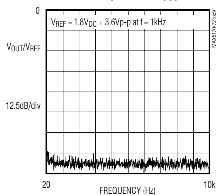
REFERENCE FEEDTHROUGH
