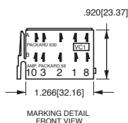
VC1 CONNECTOR HOUSING
