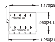
VCH CONNECTOR HOUSING
