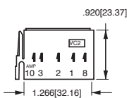
VC2 CONNECTOR HOUSING (For AMP terminals only)
