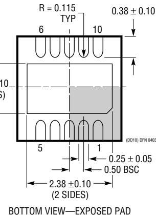
BOTTOM VIEW—EXPOSED PAD
