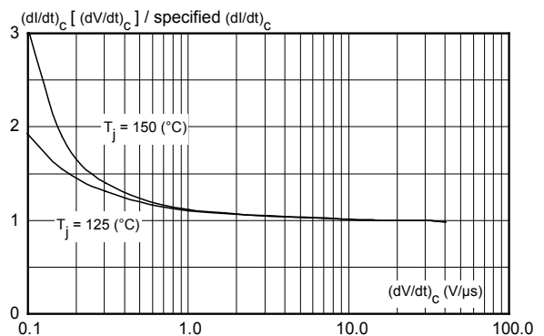
Figure 12. Relative variation of critical rate of decrease (di/dt)_c of main current versus reapplied (dV/dt)_c (maximum values)
