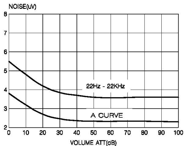
Figure 2: Noise vs. volume setting
