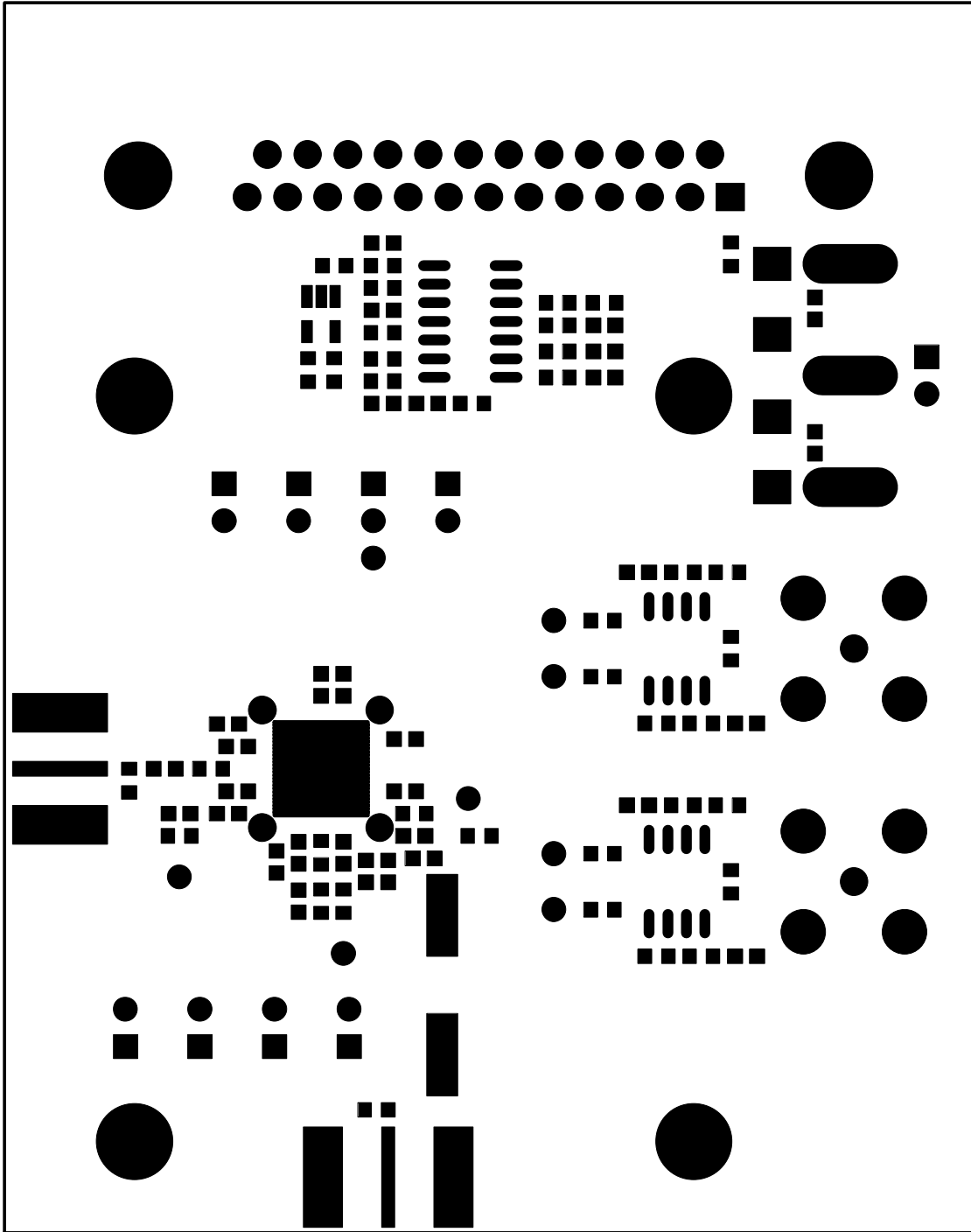
Figure 5. MAX2112 EV Kit PCB Layout—Top Soldermask
