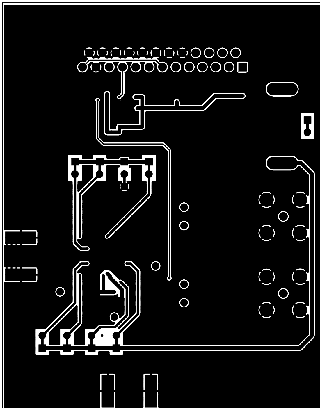
Figure 4. MAX2112 EV Kit PCB Layout—Bottom
