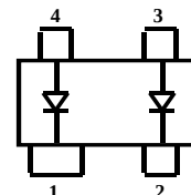
Unconnected Pair MA4E1338E-1068T
