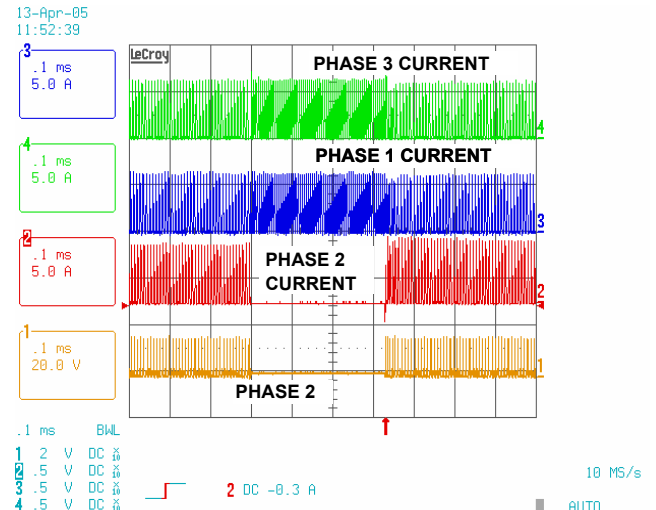
FIGURE 32. ISL6260C, INDUCTOR CURRENT WAVEFORM WITH PHASE ADDING AND DROPPING IN DCM OR DEEPER SLEEP MODE
