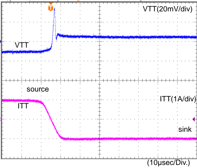
Figure 2. DDR2 (-1A→1A)
