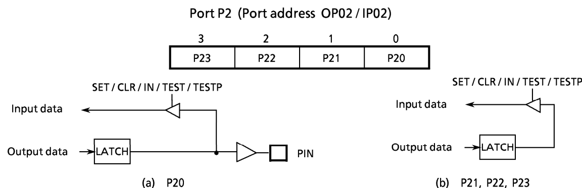
Figure 2-1. Port P2
