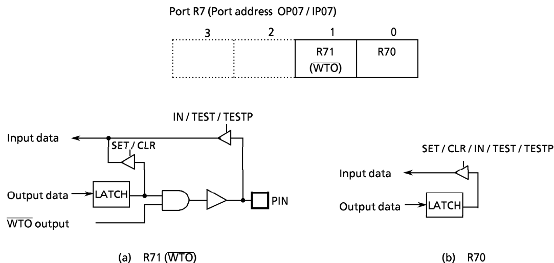
Figure 2-3. Port R7
