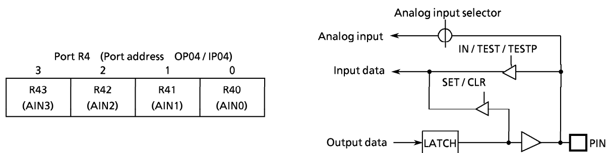
Figure 2-2. Port R4
