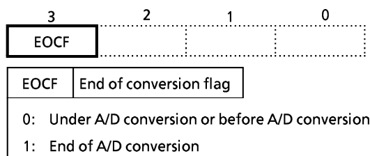
Figure 2-9. A/D converter status register
