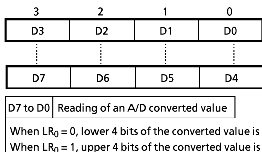
Figure 2-10. A/D converted value register
