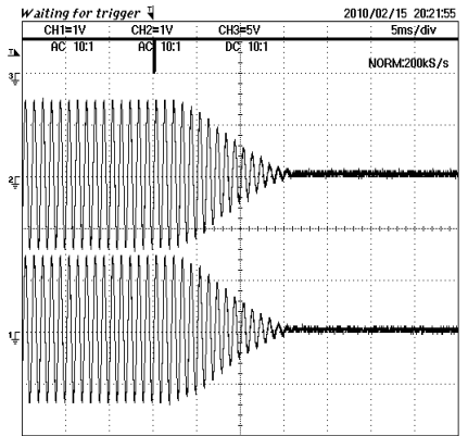
Figure 16. Advanced Switch 2
