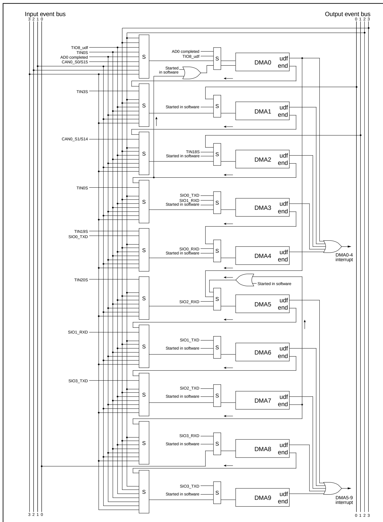
Figure 13. Block Diagram of MJT (3/3)
