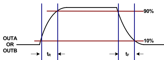
FIGURE 4. RISE/FALL TIMES
