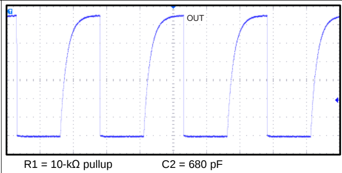
Figure 20. 10-kHz Switching Magnetic Field
