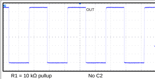
Figure 19. 10-kHz Switching Magnetic Field
