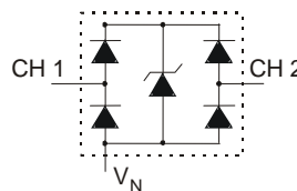
Device Schematic
