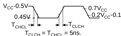
Figure 55. Clock Signal Waveform for I_{CC} Tests in Active and Idle Modes
