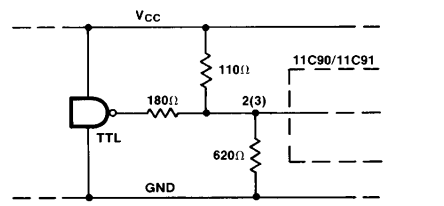
FIGURE 6. Faster Low Impedance TTL to ECL Interface
