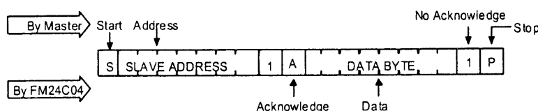
Figure 8 Sequential Read
