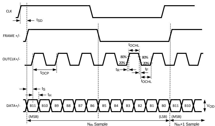
Figure 2. LVDS Output Timing
