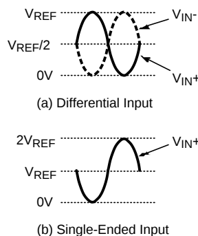
Figure 34. Expected Input Signal Range
