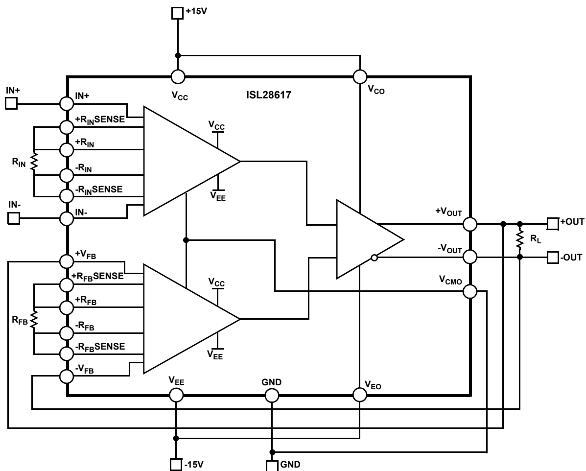
FIGURE 3. SIMPLIFIED BLOCK DIAGRAM
