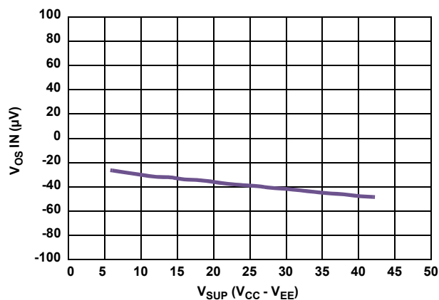
FIGURE 15. V_{OS IN} vs SUPPLY VOLTAGE ( V_{CC} - V_{EE} )
