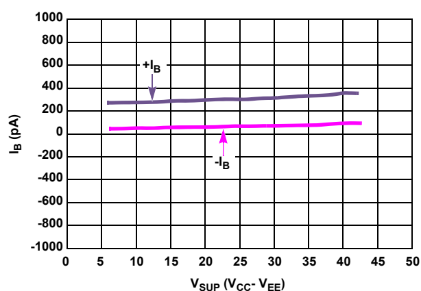
FIGURE 13. I_B vs SUPPLY VOLTAGE ( V_{CC} - V_{EE} )
