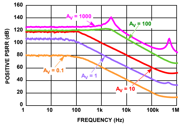
FIGURE 23. POSITIVE PSRR V_{EE} AND V_{CC} ( R_F = 121k )
