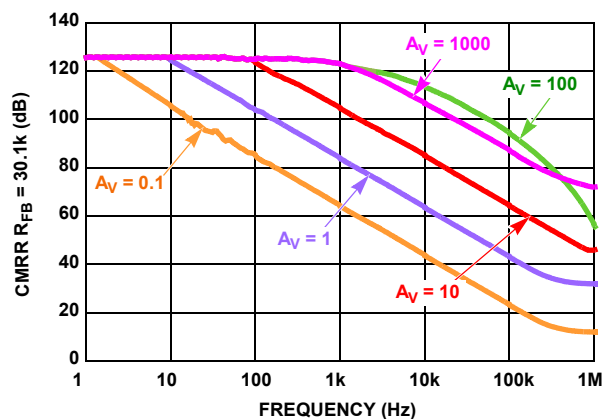
FIGURE 29. CMRR R_F = 30.1k
