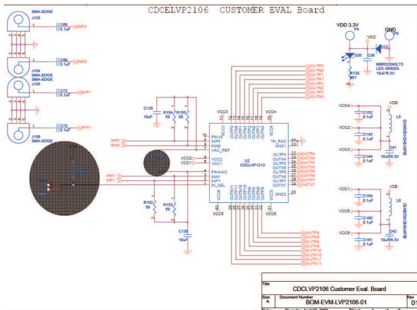
Figure 2. CDCLVP2106EVM—Schematic
