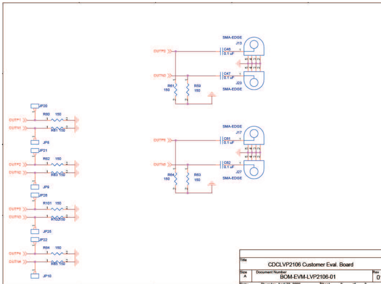
Figure 3. CDCLVP2106EVM—Schematic
