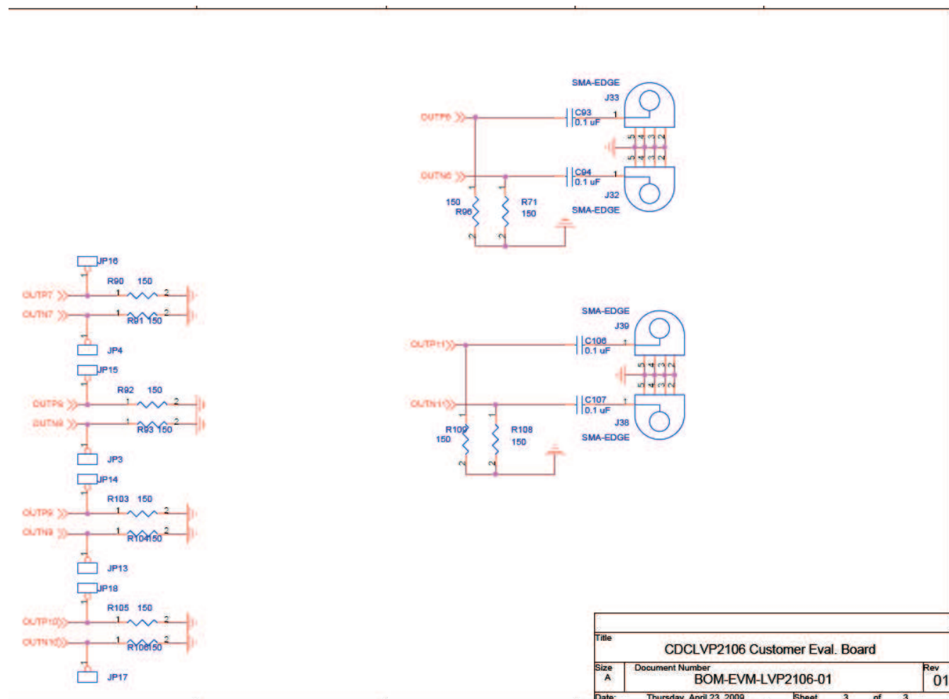
Figure 4. CDCLVP2106EVM—Schematic
