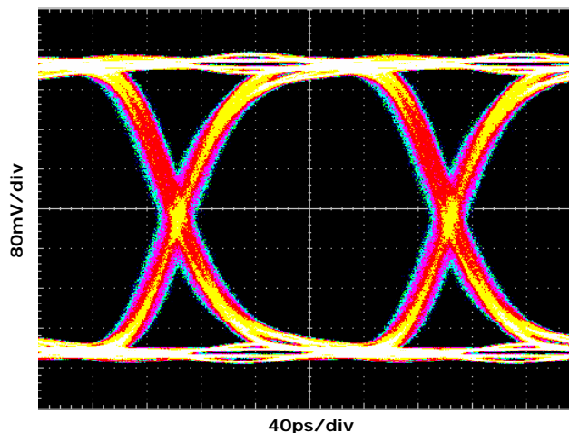
FIGURE 5. QLx4600-SL30 OUTPUT AFTER 20m OF 24AWG TWIN-AXIAL CABLE (CABLE A), 5Gb/s
